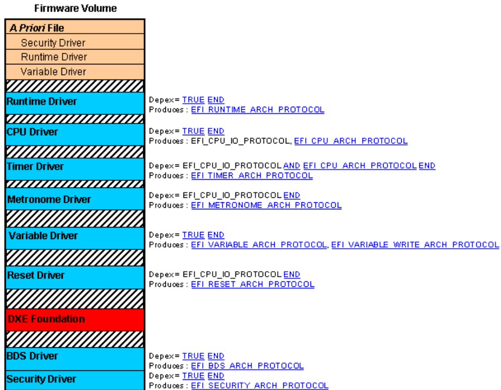
Figure 10.2. Sample Firmware Volume
